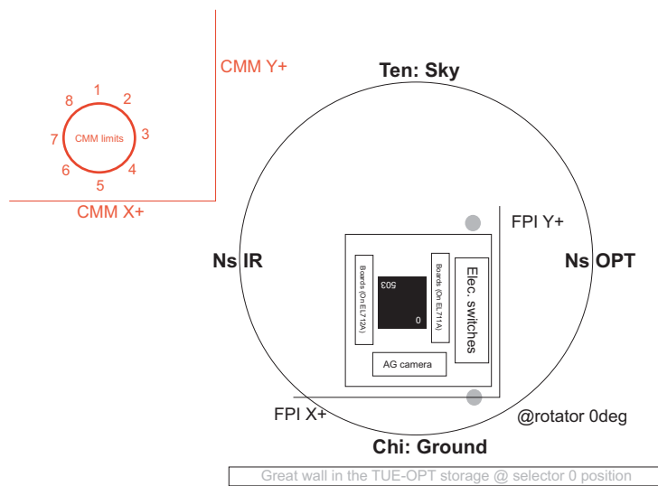
Figure 6: The relation between the Echidna unit and the PIR/CMM unit at rotator angle of 0 degree. ??? THE CONFIGURATION NEED TO BE CHECKED !!!
