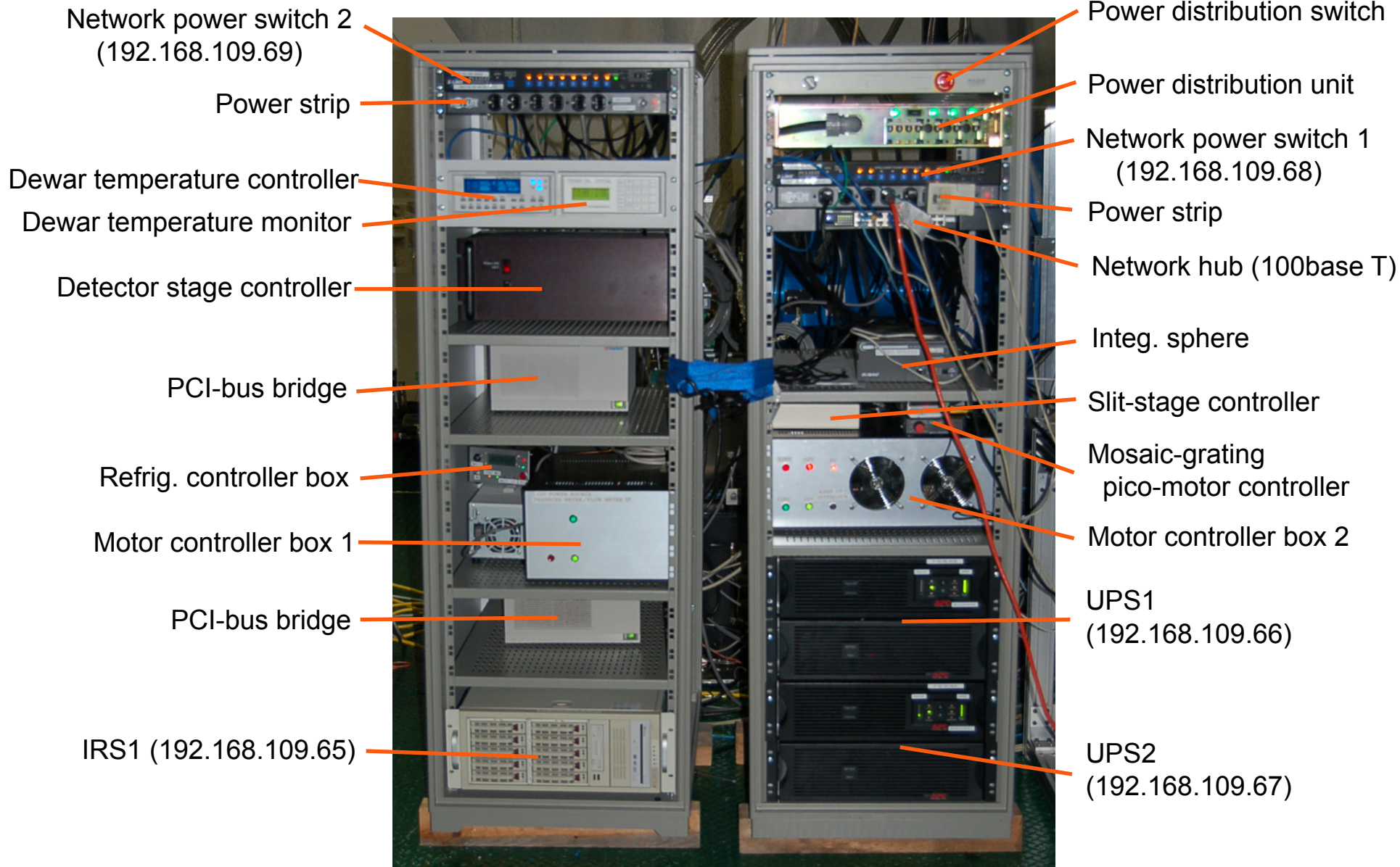
Rack 2
