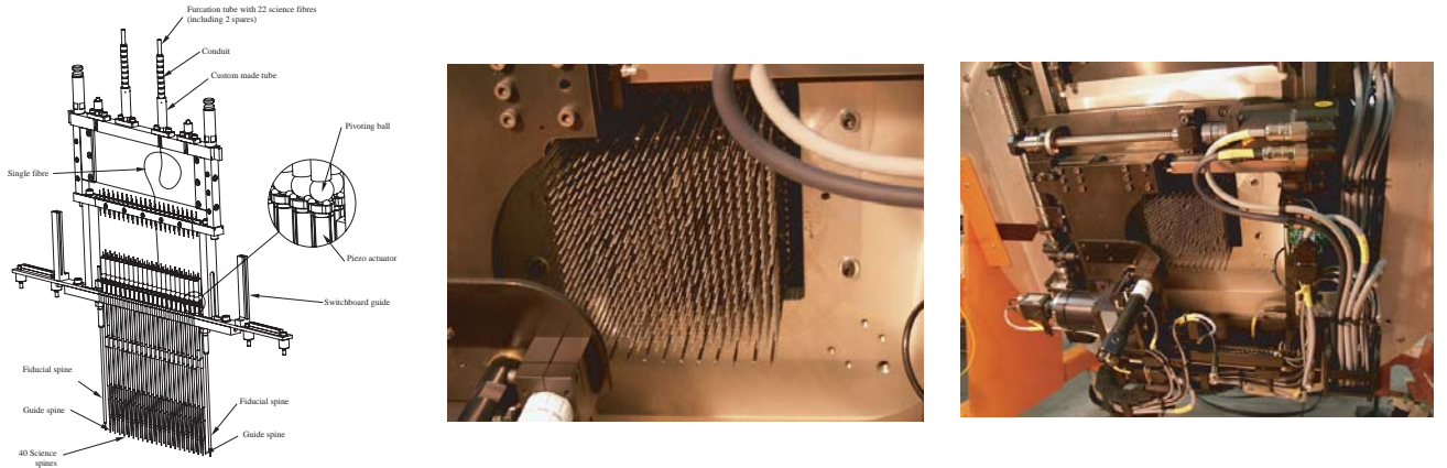
Figure 1. Left) drawing of one module of the fiber positioner from Fig. 4 of Ref6. One module has 20 \times 2 science-fibers and 2 guide-bundles at both ends of the module. Science-fibers are 100\mu\text{m} diameter core fiber, and guide-bundles are bundles of 7 50\mu\text{m} -core fibers with 80\mu\text{m} spacing, which corresponds to 0.96'' at the focal plane. A fiber is attached to a carbon-fiber tubing, called “spine”, with a pivoting ball and a tungsten counter weight. The pivoting ball is sitting on a three-point mount with a ring magnet at the top of a quadrant tube piezo actuator. Spines for the science-fibers and the guide-bundles have the same structure. Middle) close up view of the focal plane. 12 modules of the 40 science-fibers cover the FoV. 400 science-fibers within the 30' diameter FoV are connected to the spectrographs. The spacing between neighboring spines is 7\text{mm} . Each spine is designed to be able to reach the home positions the 6 neighboring spines. Right) structure of the Echidna unit around the focal plane. The positions of the tips of the fibers are measured with the fiber camera of the Focal Plane Imager (FPI) on the XY gantry.
