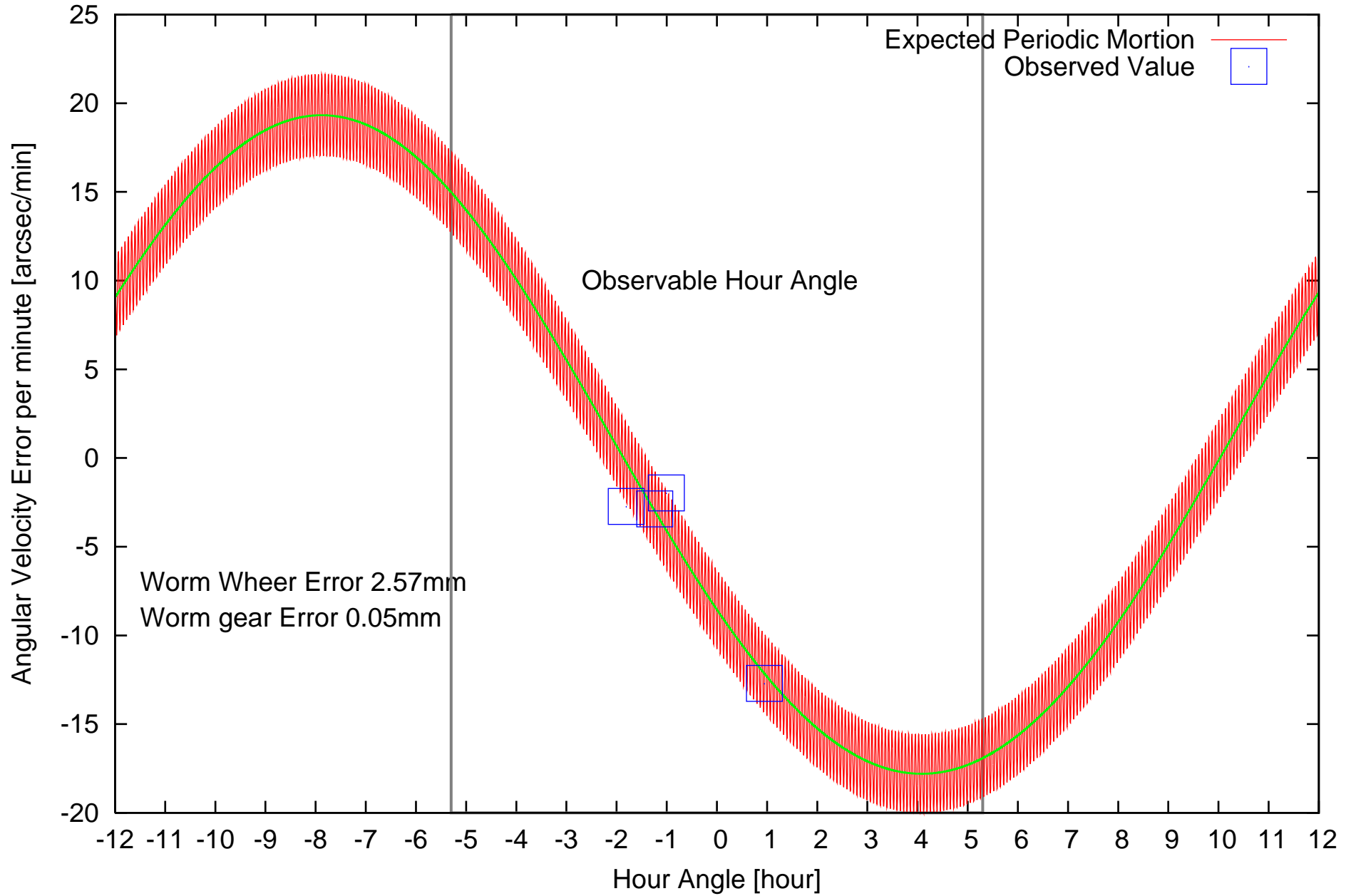
Periodic Error by Worm Wheel and Worm Gear
