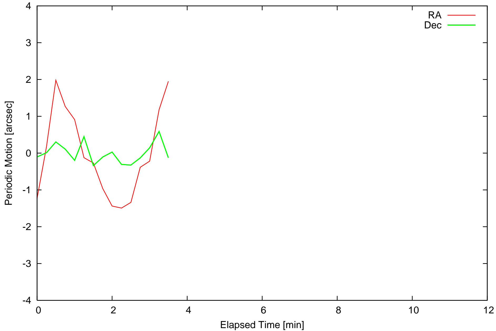
Periodic Motion (Tracking Error Cancelled) 2008-10-17T10:03:12(UTC)
