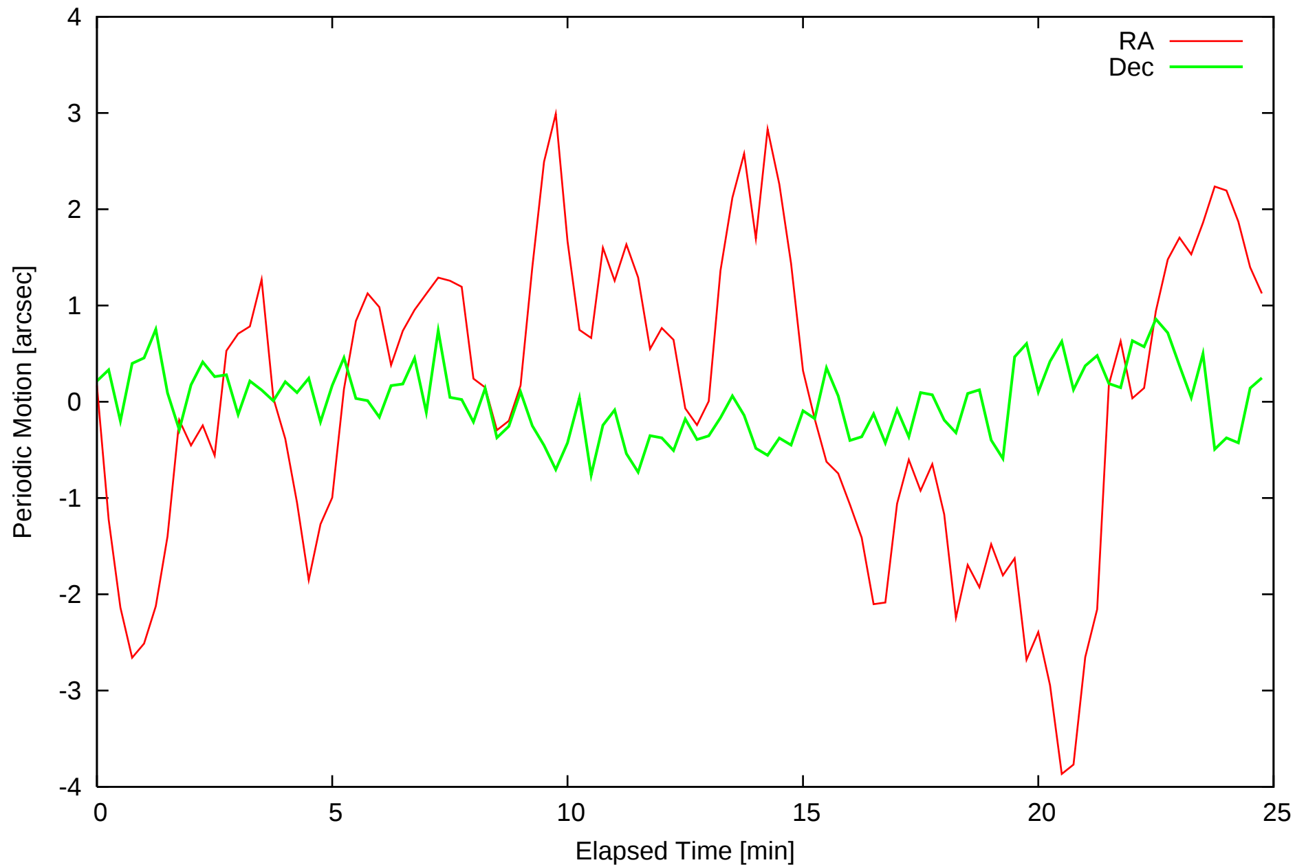
Periodic Motion (Tracking Error Cancelled) 2008-10-21T09:14:26(UTC)
