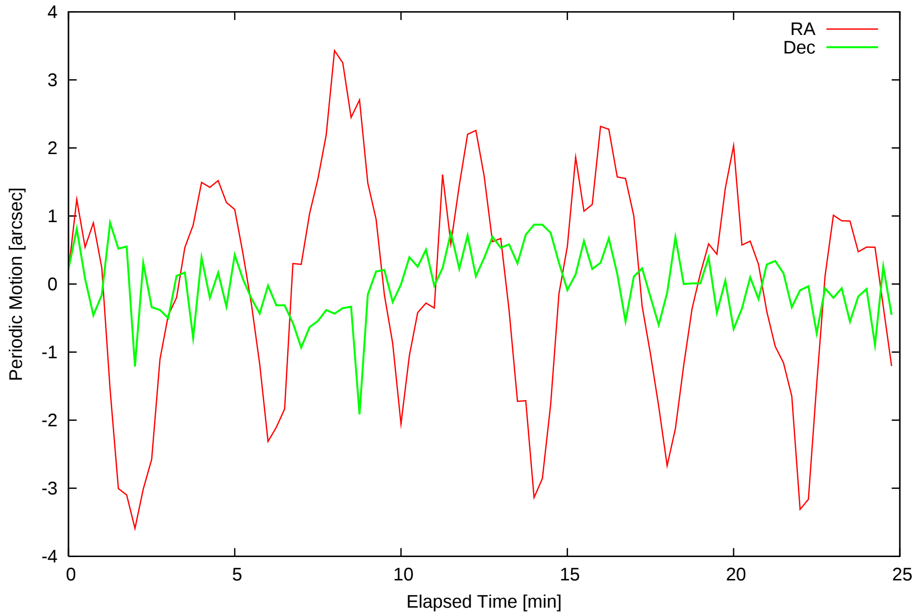
Periodic Motion (Tracking Error Cancelled) 2008-10-21T10:20:57(UTC)
