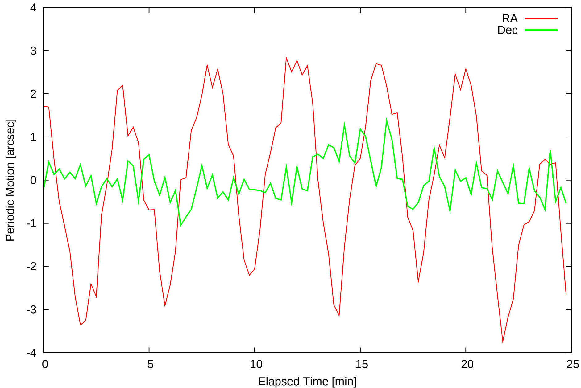
Periodic Motion (Tracking Error Cancelled) 2008-10-21T09:41:24(UTC)
