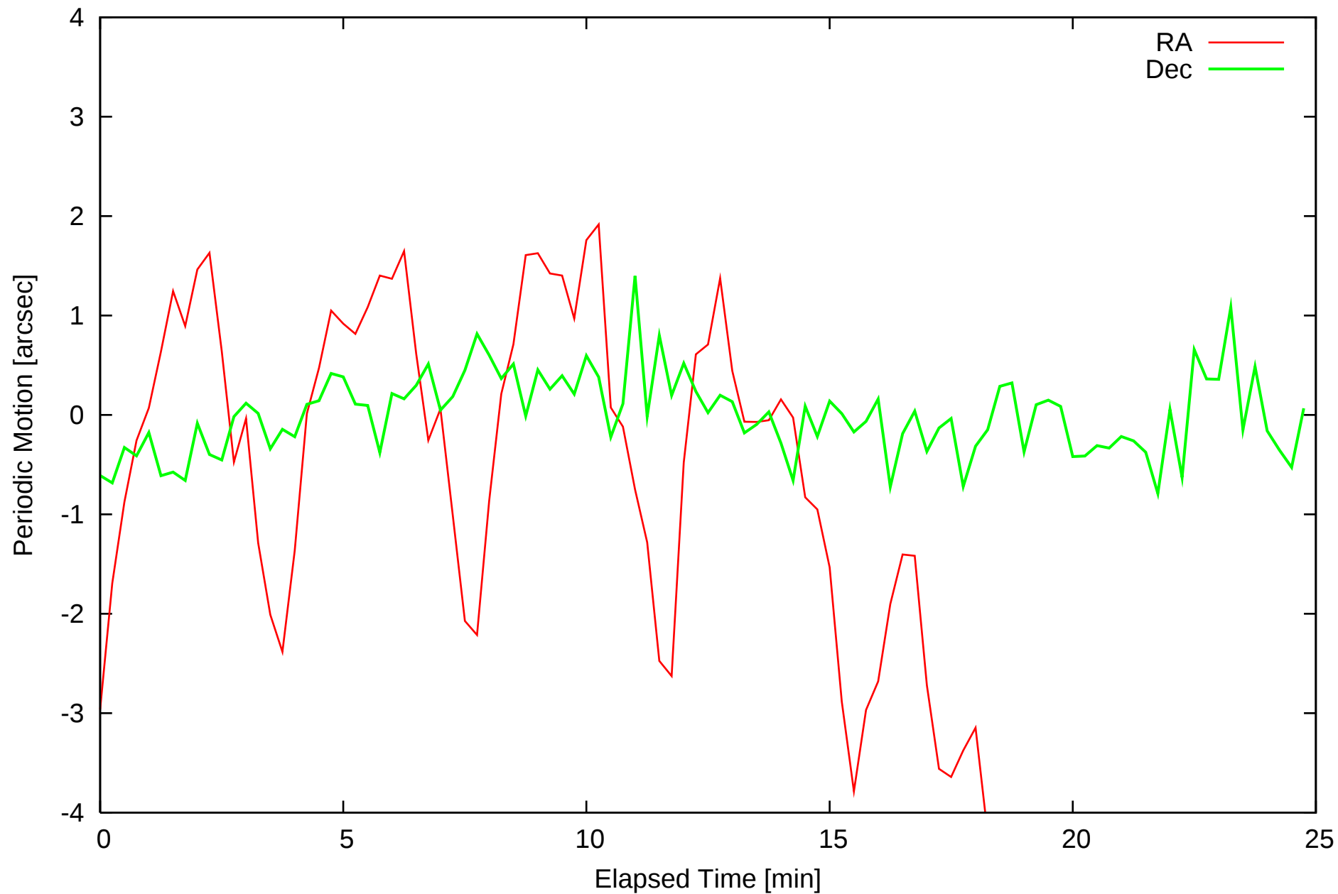
Periodic Motion (Tracking Error Cancelled) 2008-10-21T10:47:19(UTC)
