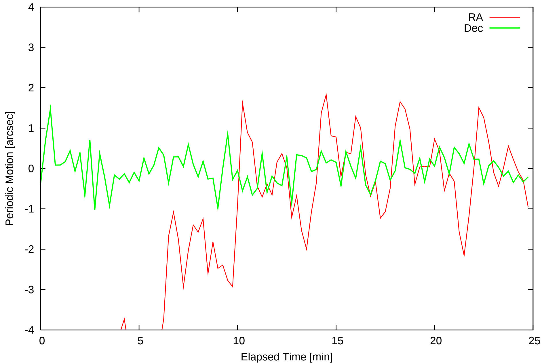
Periodic Motion (Tracking Error Cancelled) 2008-10-21T11:13:15(UTC)
