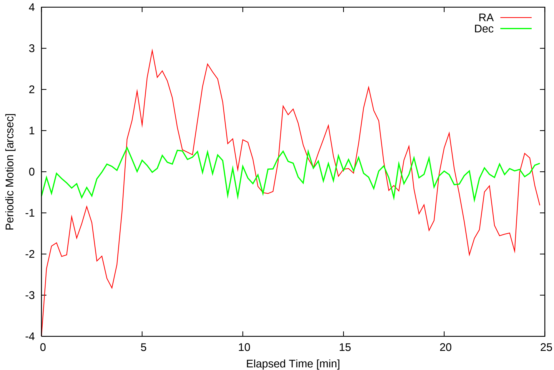
Periodic Motion (Tracking Error Cancelled) 2008-10-21T08:37:59(UTC)
