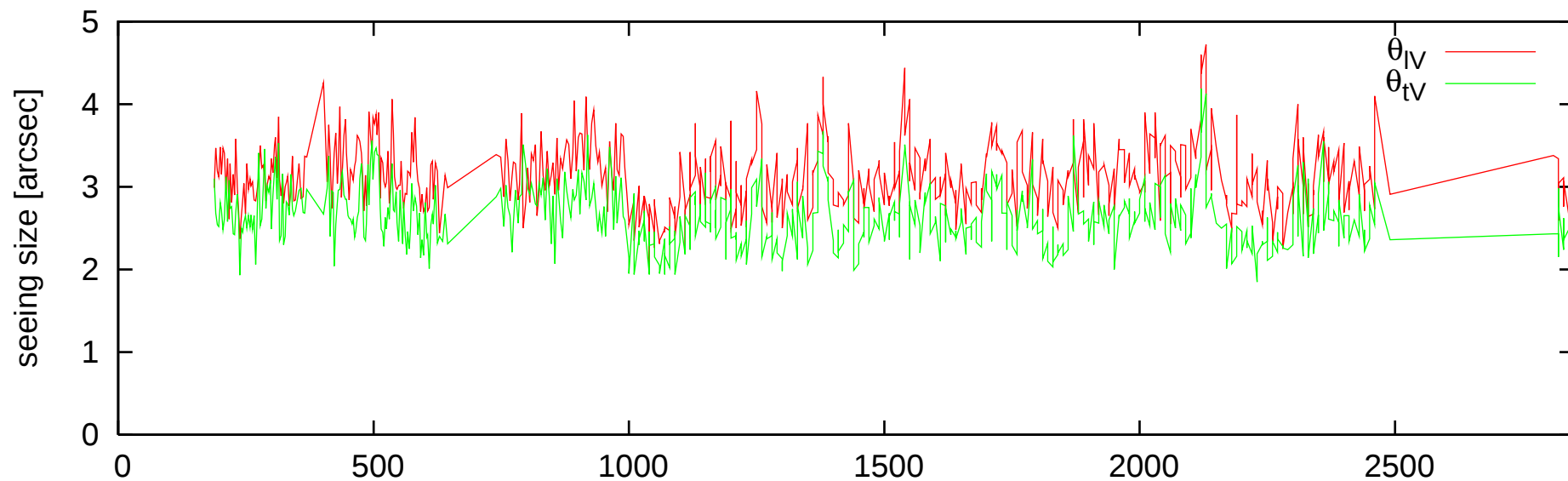
DIMM observation at RIKUBETHU 2008/02/14 19h54m-20h38m using \alpha -Aur
