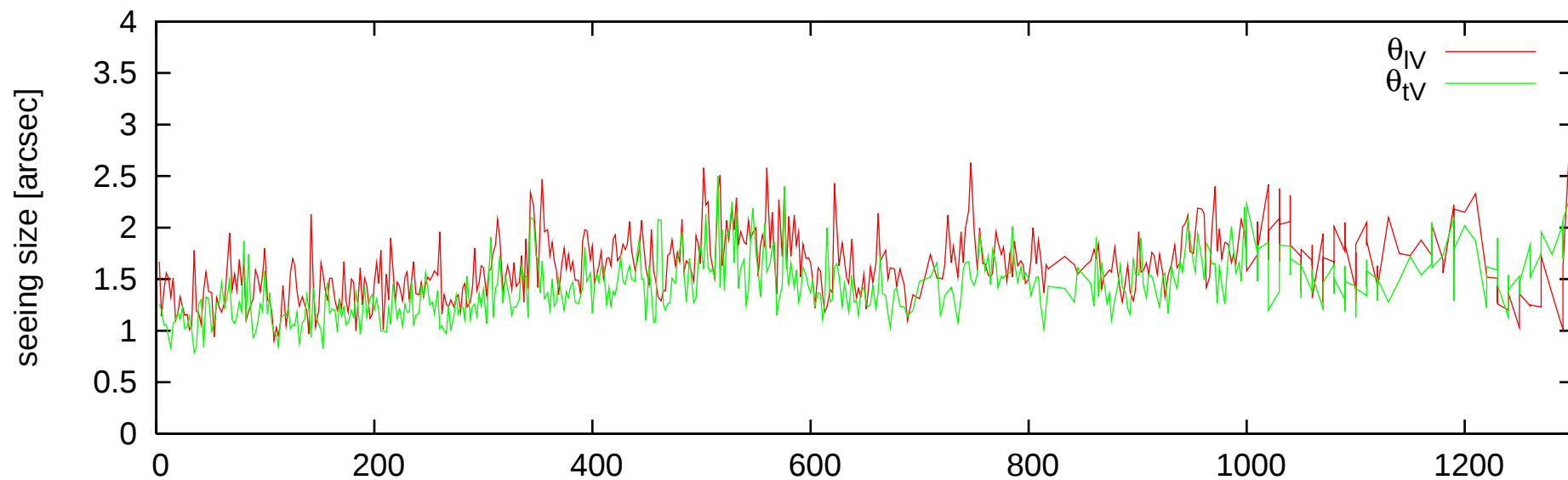
DIMM observation at RIKUBETSU 2008/02/11 00h00m-00h22m using \beta -Gum
