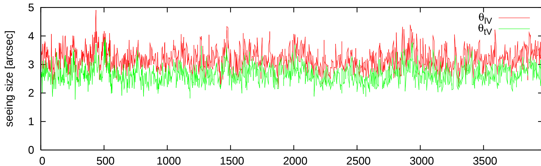
DIMM observation at RIKUBETHU 2008/02/14 20h38m-21h45m using \alpha -Aur
